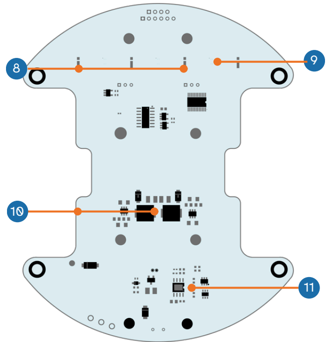
• Figure 2: Lower base, rear face
