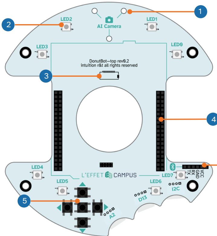
• Figure 3: Upper base, front face
