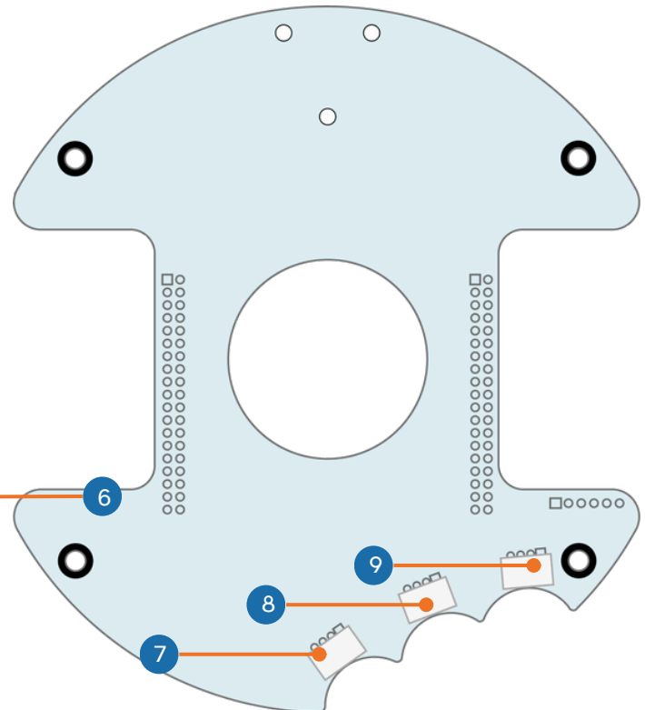
• Figure 4: Upper base, rear face
