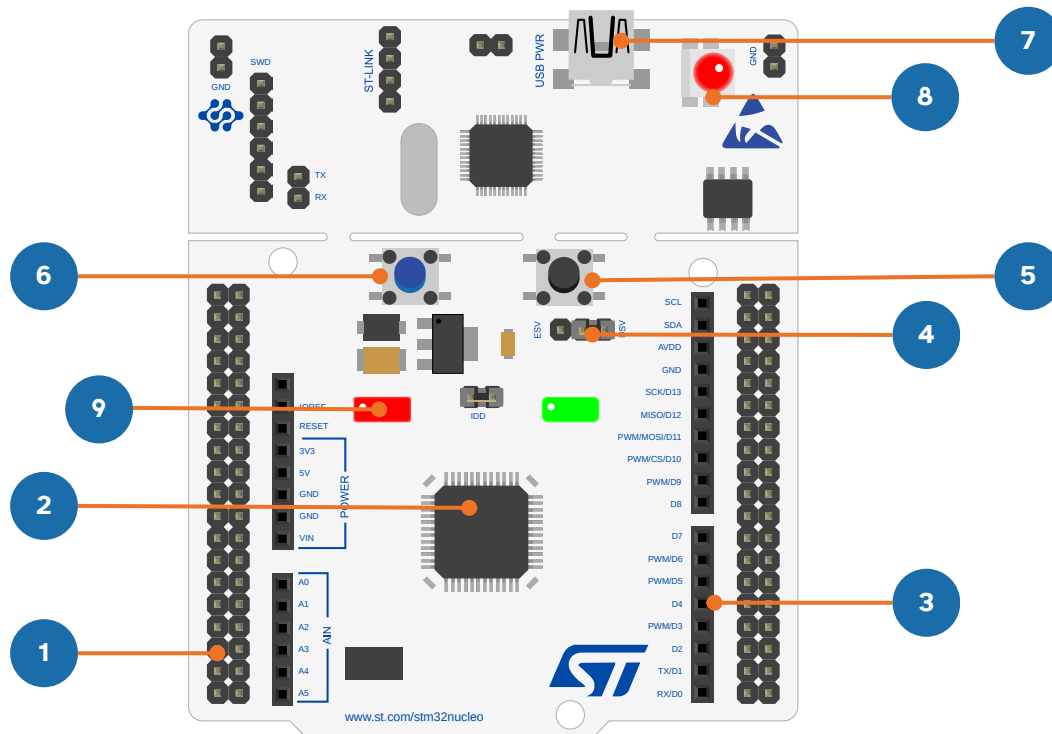
• Figure 5: NUCLEO-L476RG (front panel)
