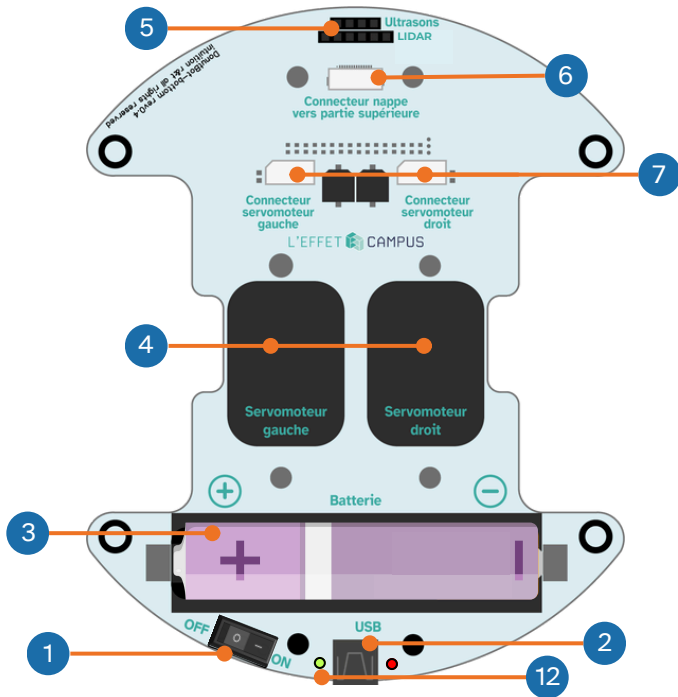
• Figure 1: Lower base, front face
